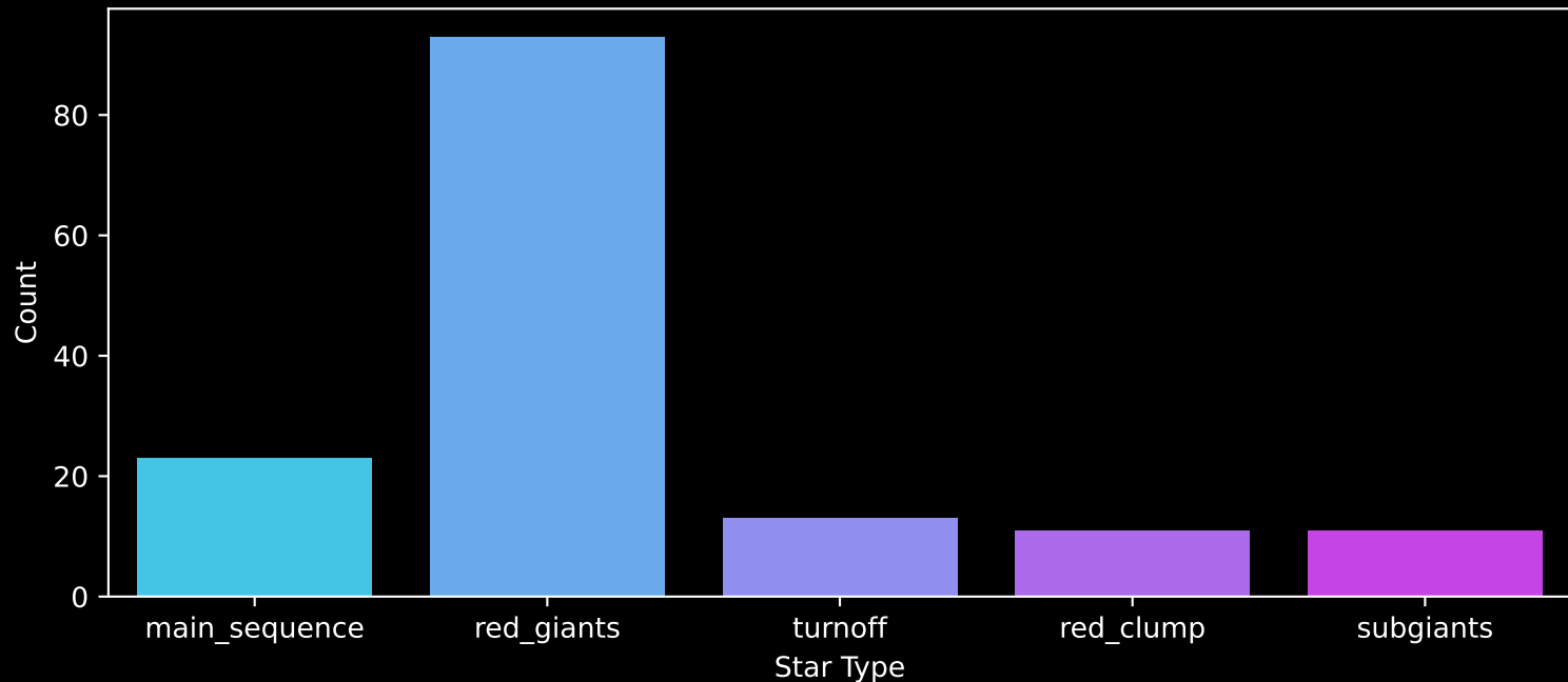
APOGEE DR17 Field: [K2_C7_012-21] Count plot of Star Type
