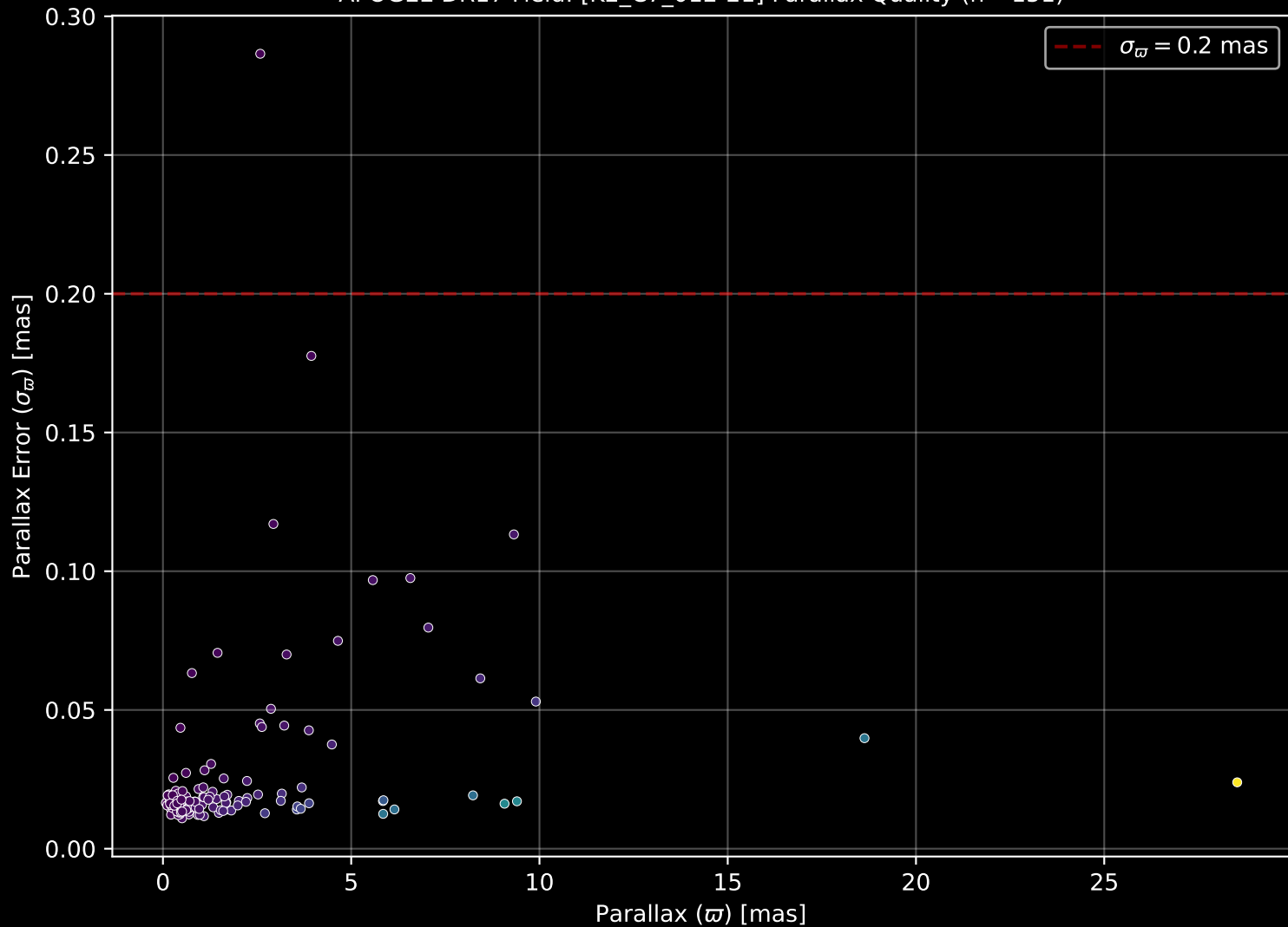
APOGEE DR17 Field: [K2_C7_012-21] Parallax Quality (n= 151)
