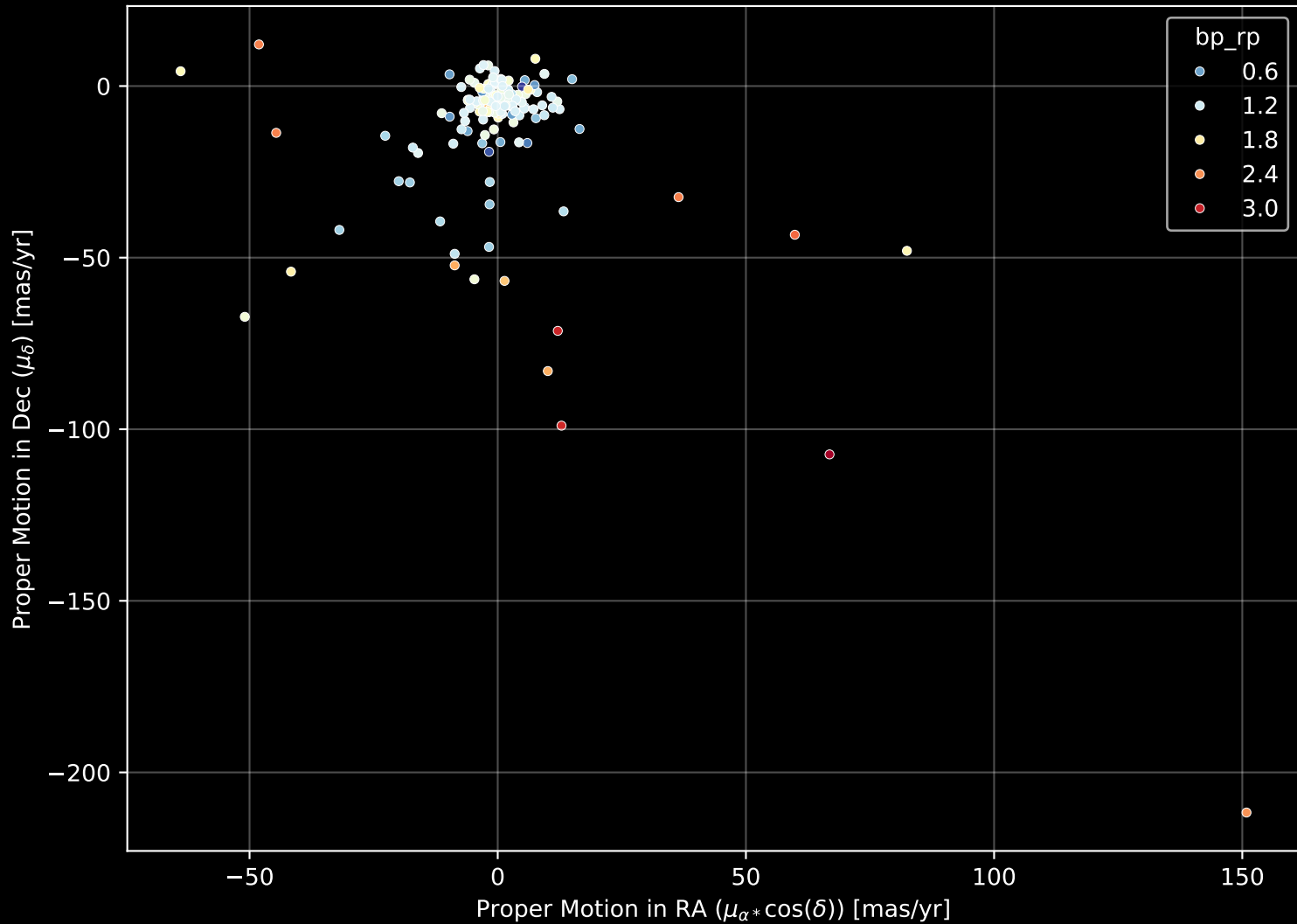
APOGEE DR17 Field: [K2_C7_012-21] Proper Motion Diagram (n= 151)
