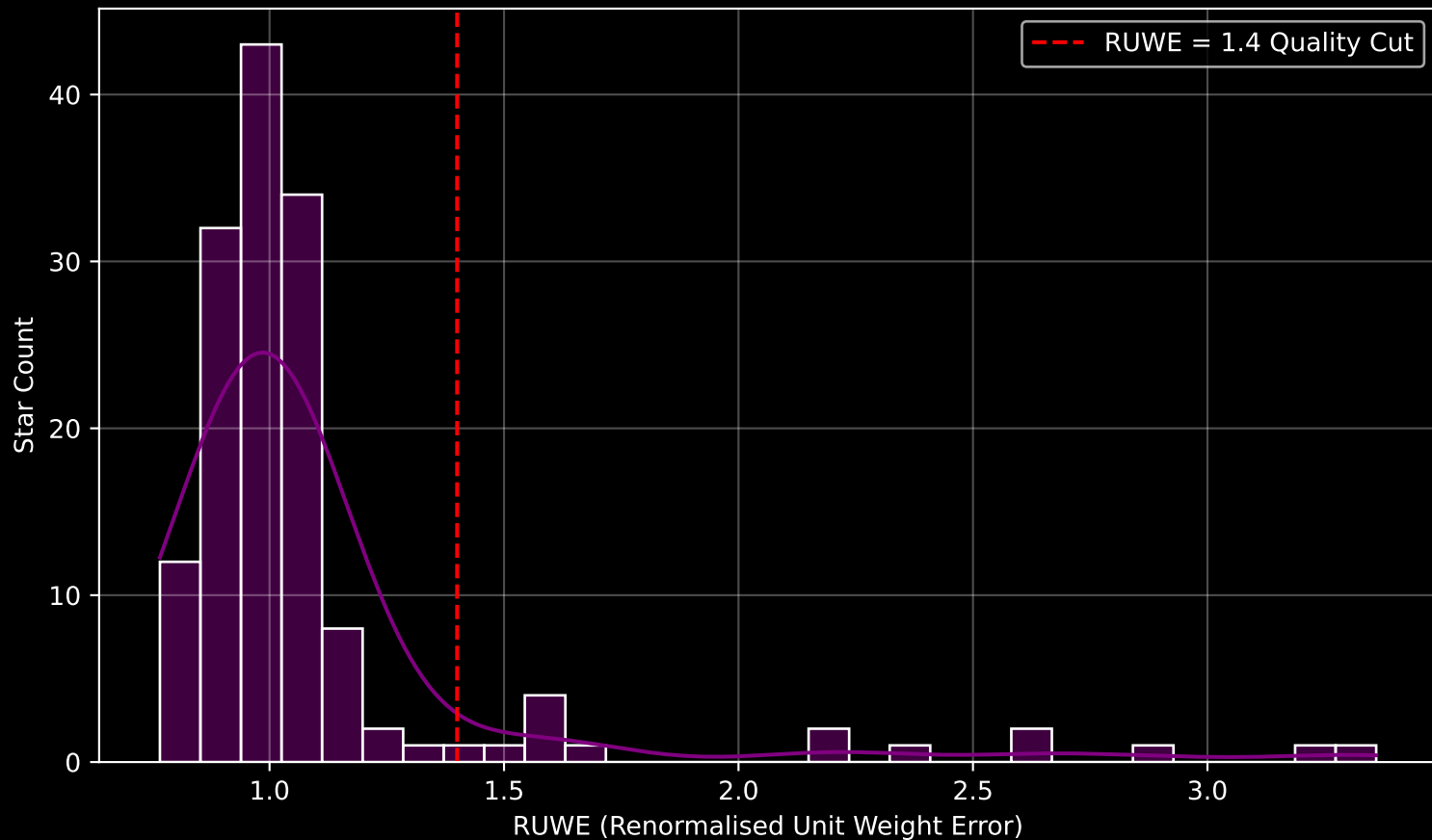
GAPOGEE DR17 Field [K2_C7_012-21] RUWE Distribution (n= 147)
