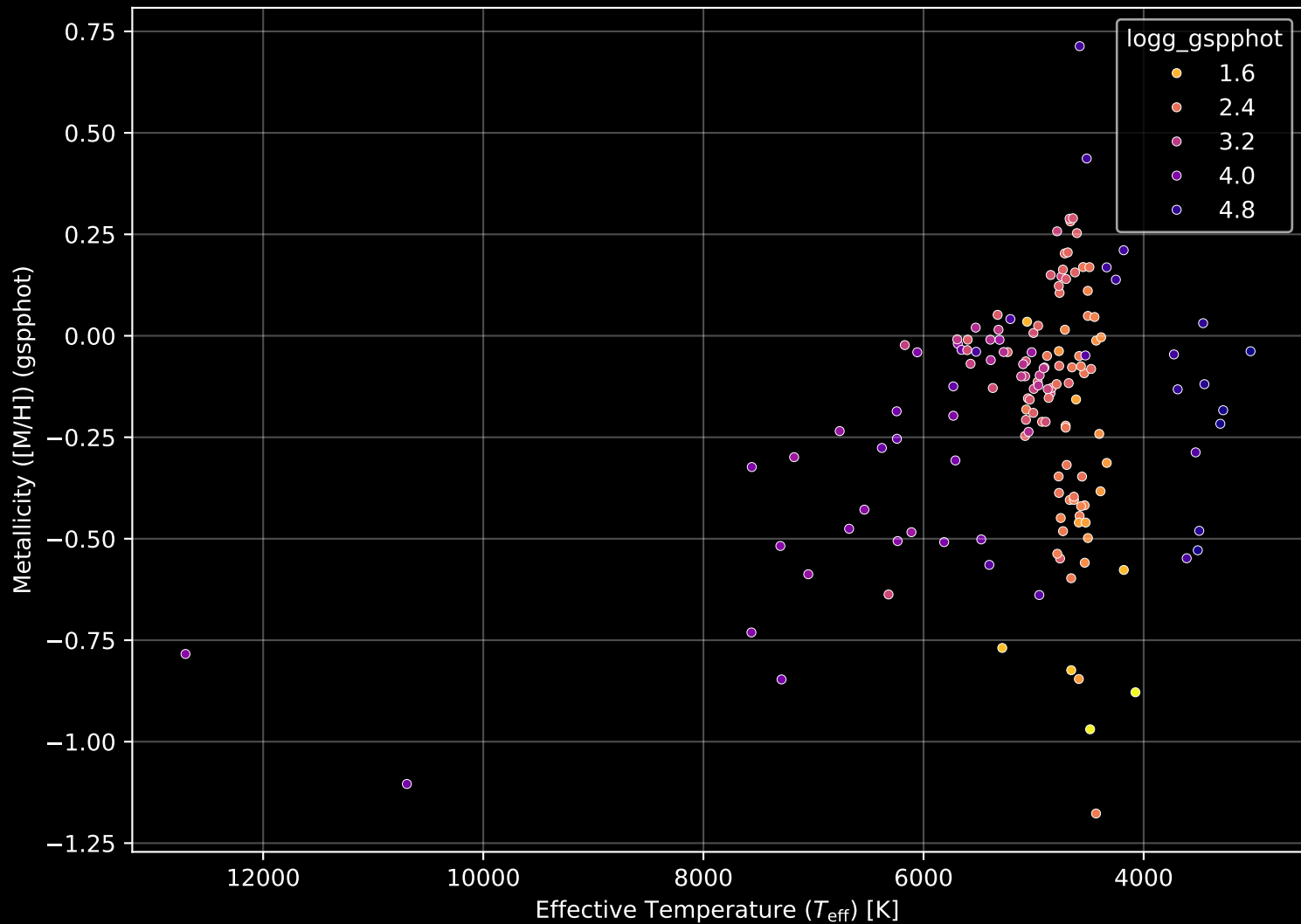
APOGEE DR17 Field: [K2_C7_012-21] Stellar Population Parameters (n= 151)
