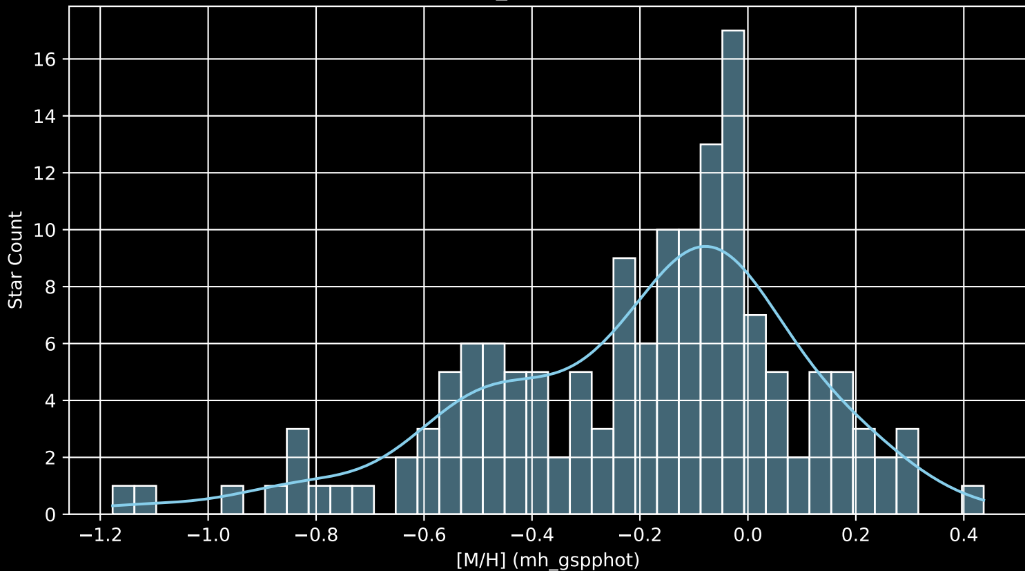
APOGEE DR17 Field: [K2_C7_012-21 [M/H] (mh_gspphot) (n= 150)
